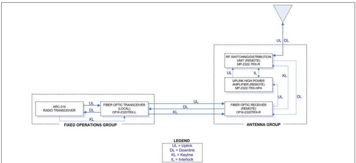
Tactical Radio Deployment - Function Block Diagram
